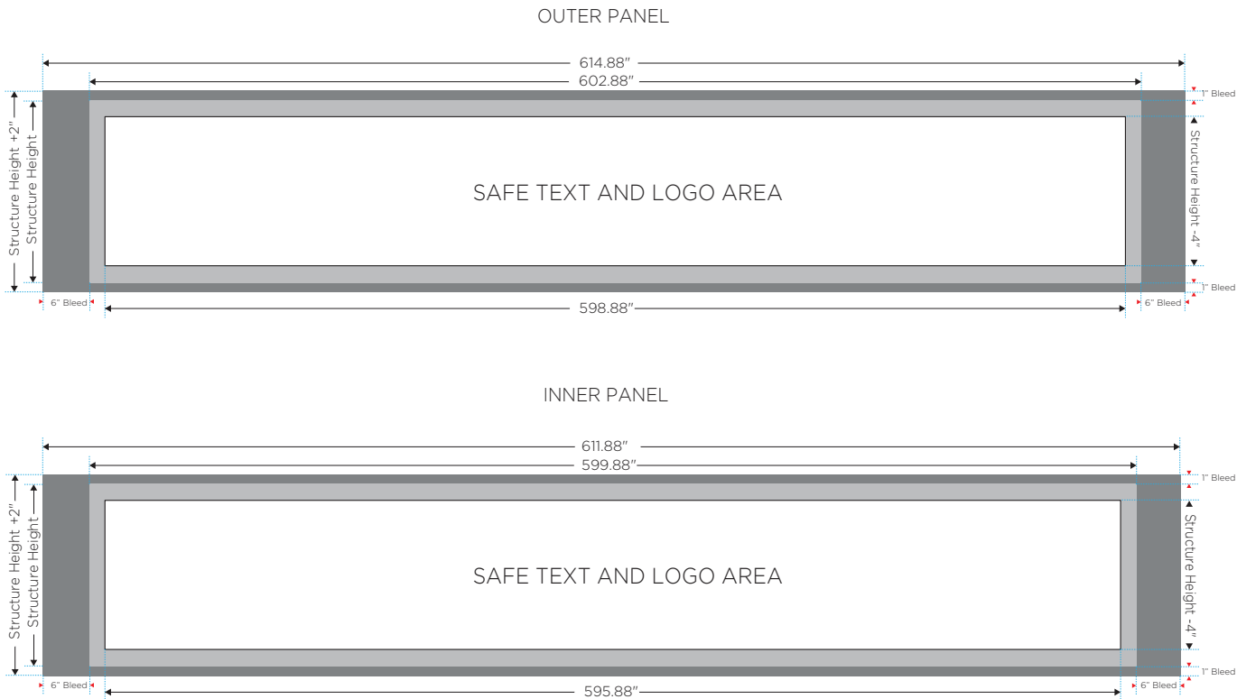
16' dia. PILLOW FIT HALO GRAPHIC SIZES:
